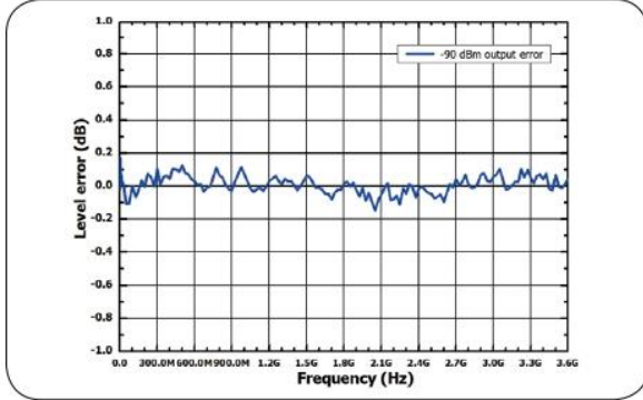
Measured at -90 dBm, level error vs. frequency
