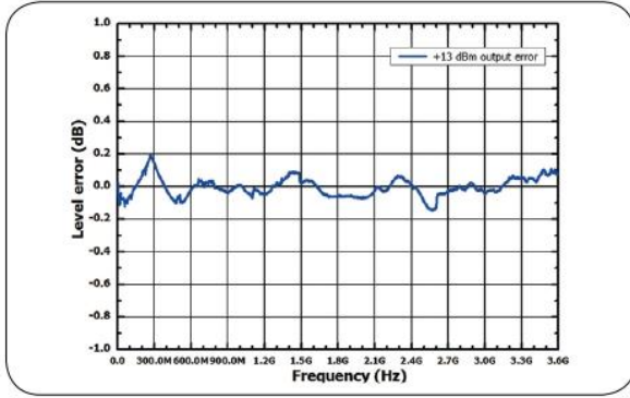
Measured at +13 dBm, level error vs. frequency
